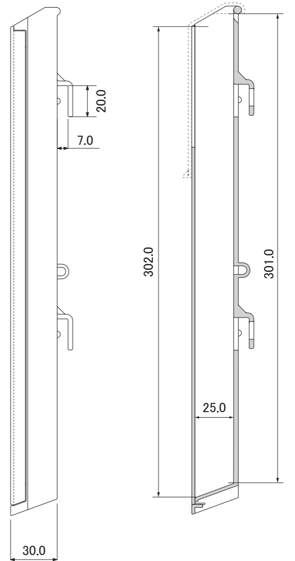
SECT B-B'
