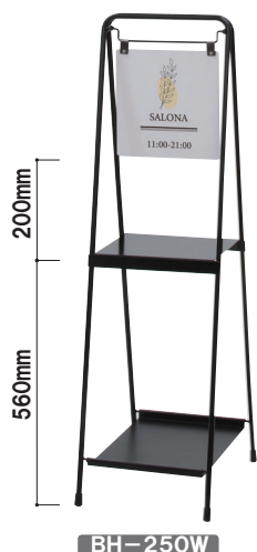
BH-250W
